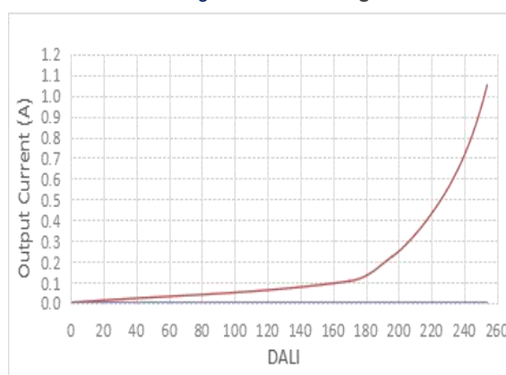
Logarithmic dimming
