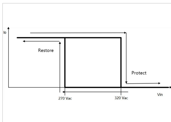
Schematic diagram of input overvoltage protection
