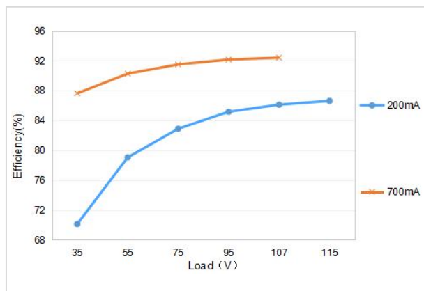
Working Curve
