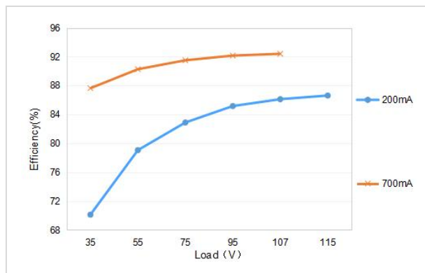
Efficiency Curve
